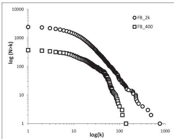
Fig. 1: Cumulative degree distributions (log-log plot) of the smallest (FB_400) and the largest (FB_2k) networks examined. The networks have 372 and 2220 nodes.
